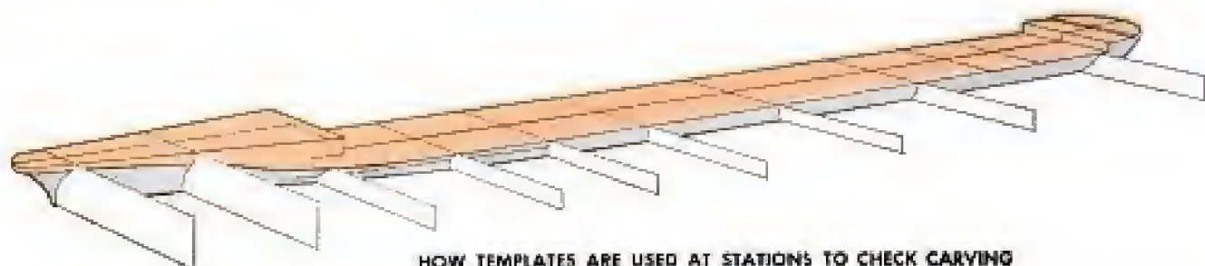
HOW TEMPLATES ARE USED AT STATIONS TO CHECK CARVING
